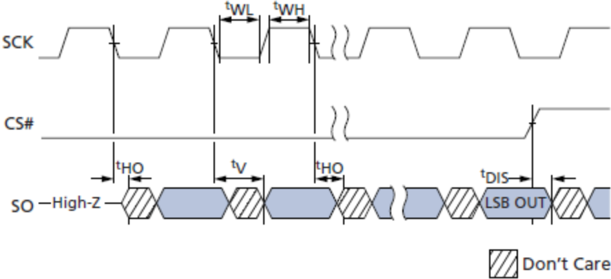
Serial Output Timing
