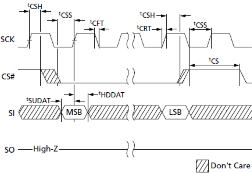
Serial Input Timing
