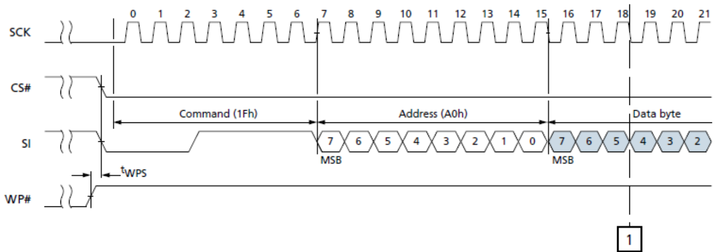
WP# Timing
